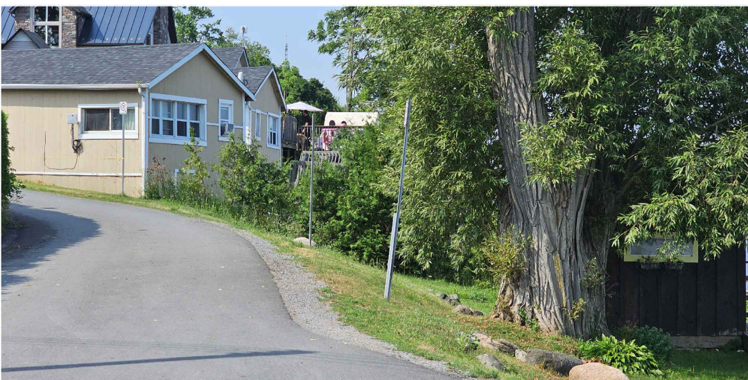
VIEW OF EXISTING SLOPE ON SOUTH END OF SITE FROM INTERSECTION OF FRONT STREET AND RAILWAY ROAD
