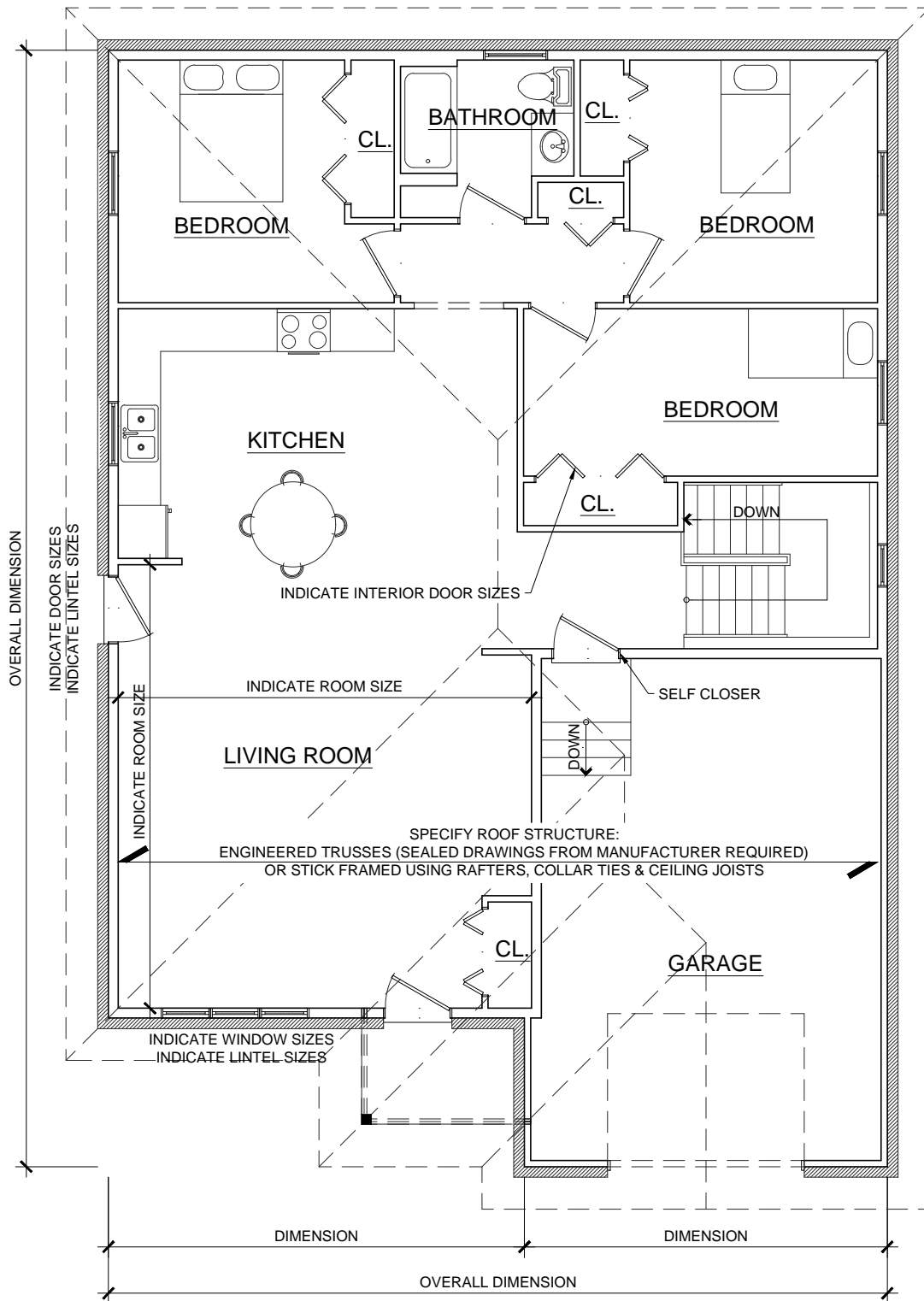
SAMPLE HOUSE FLOOR PLAN
